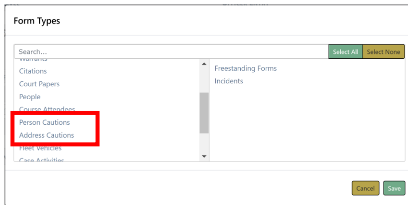
FIGURE 32: CUSTOM FORMS - NEW FORM TYPES FOR PERSON AND ADDRESS CAUTIONS
